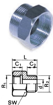
ANI nipple female x male threads, galvanized steel
