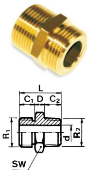
ANA nipple with two male threads, brass
