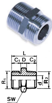
ANA nipple with two male threads, galvanized steel
